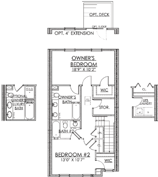
2 BEDROOMS/ 2 BATH
